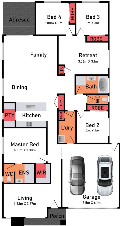
FLOOR PLAN
